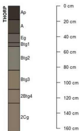
Figure 11. Figure 6. Profile sketches of soil series associated with Ponded Upland Depression Sedge Meadow.
