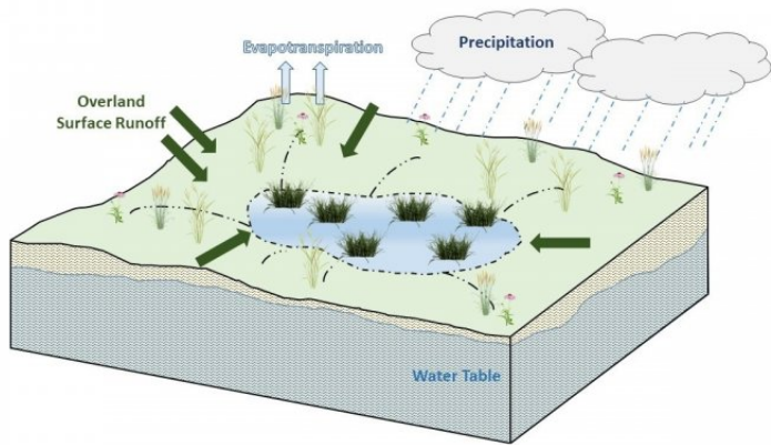
Figure 10. Figure 5. Hydrologic cycling in Ponded Upland Depression Sedge Meadow ecological site.
