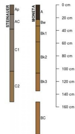
Figure 9. Figure 6. Profile sketches of soil series associated with Calcareous Till Upland Prairie.
