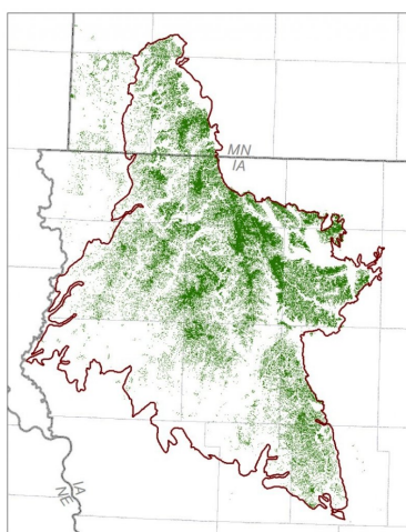
Figure 2. Figure 1. Location Wet Upland Sedge Meadow ecological site within MLRA 107A.
