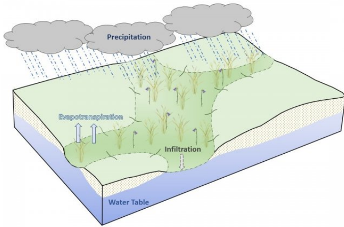
Figure 8. Figure 5. Hydrologic cycling in Wet Upland Sedge Meadow ecological site.
