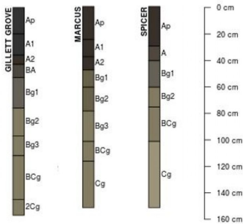
Figure 9. Figure 6. Profile sketches of soil series associated with Wet Upland Sedge Meadow.
