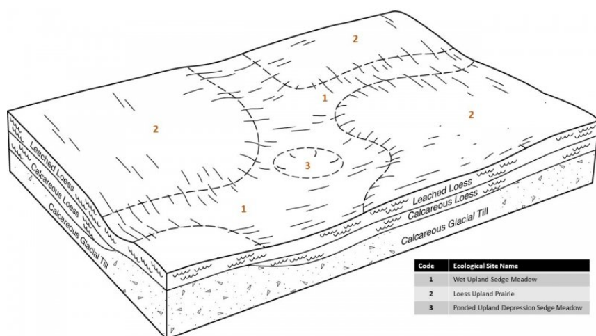
Figure 3. Figure 2. Representative block diagram of Wet Upland Sedge Meadow and associated ecological sites.
