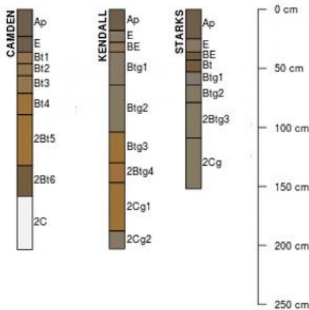
Figure 10. Figure 6. Profile sketches of soil series associated with Outwash Forest.
