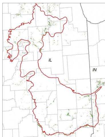
Figure 1. Location of Outwash Forest ecological site within MLRA 108A.
