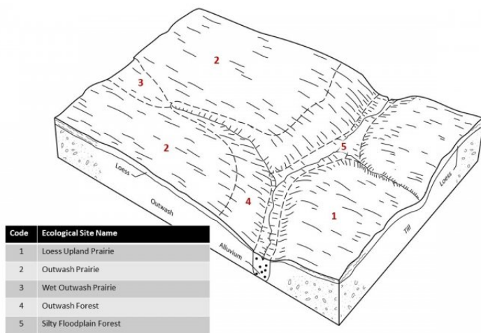
Figure 2. Figure 2. Representative block diagram of Outwash Forest and associated ecological sites.
