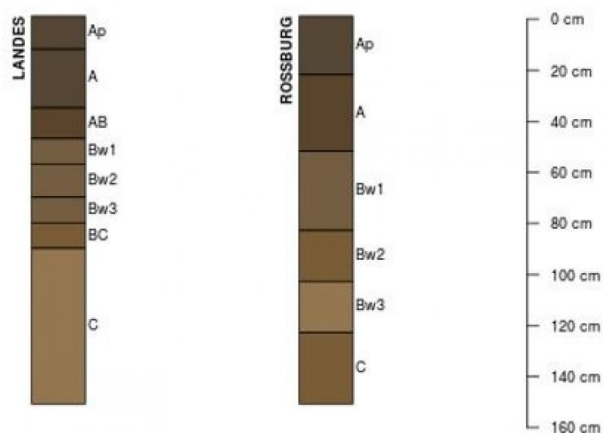
Figure 10. Figure 6. Profile sketches of soil series associated with Loamy Floodplain Forest.
