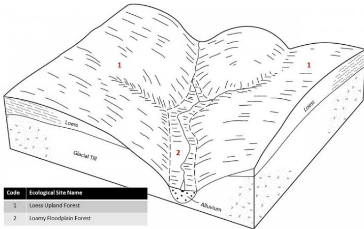
Figure 2. Figure 2. Representative block diagram of Loamy Floodplain Forest and associated ecological sites.
