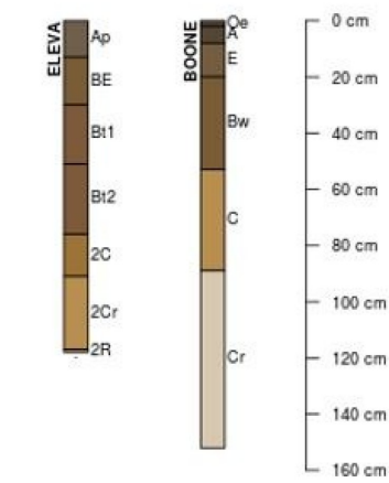
Figure 9. Figure 6. Profile sketches of soil series associated with Shallow Sandstone Backslope Glade.
