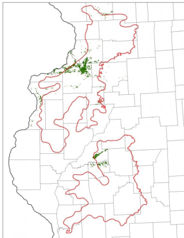
Figure 1. Location of Wet Lacustrine Prairie ecological site within MLRA 108B.
