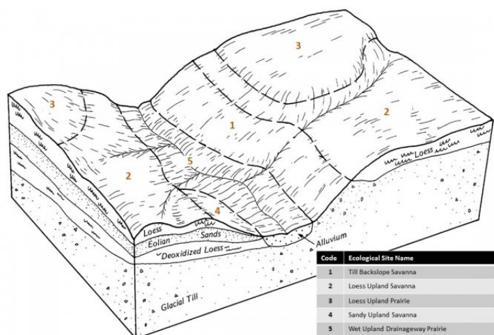
Figure 3. Figure 2. Representative block diagram of Till Backslope Savanna and associated ecological sites.
