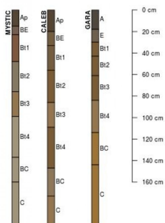
Figure 7. Figure 6. Profile sketches of soil series associated with Till Backslope Savanna.
