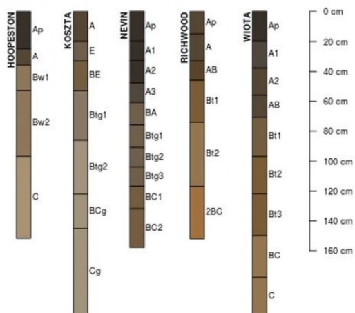
Figure 9. Figure 6. Profile sketches of soil series associated with Terrace Savanna.
