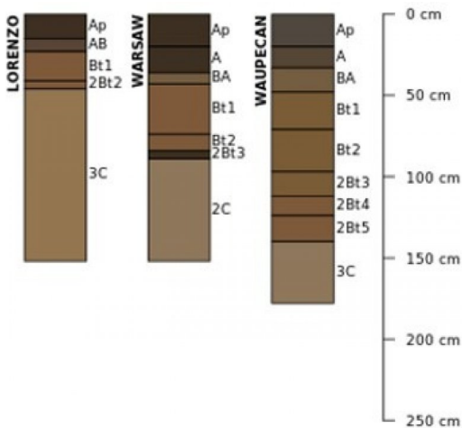
Figure 10. Profile sketches of soils series associated with Dry Glacial Drift Upland Prairie.
