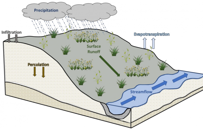
Figure 9. Hydrologic cycling in Dry Glacial Drift Upland Prairie ecological site.
