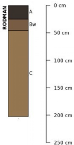
Figure 9. Profile sketches of soil series associated with Very Steep Gravel Prairie.
