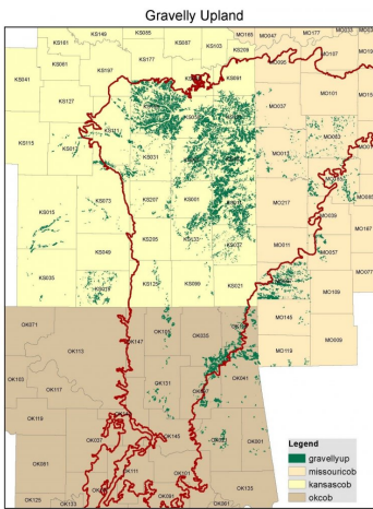
Figure 8. Spatial extent of Gravelly Upland ecological site within MLRA 112.
