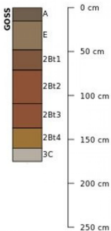
Figure 10. Profile sketches of soil series associated with Chert Exposed Backslope Woodland.
