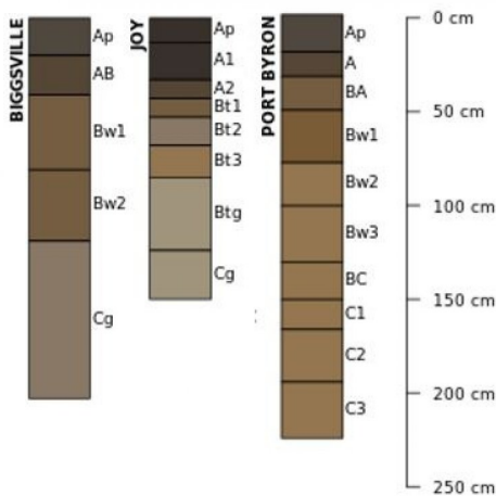
Figure 10. Profile sketches of soil series associated with Loess Upland Prairie.
