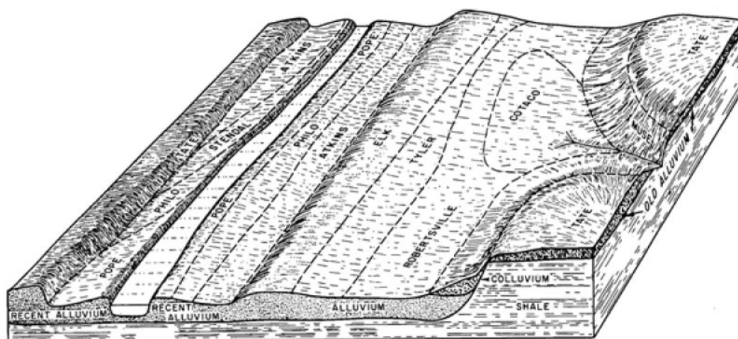
Figure 1. Block Diagram
