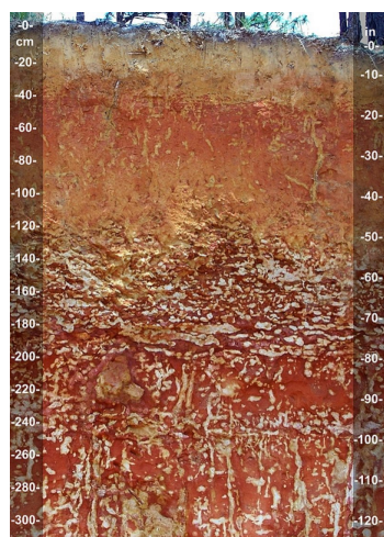
Figure 7. Profile of the Vaucluse series.
