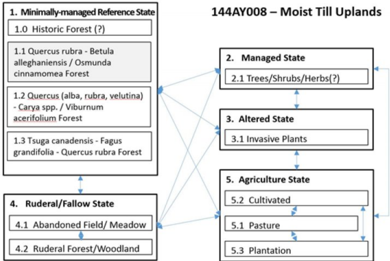
Figure 5. STM_144AY008_Moist_Till_Upland
