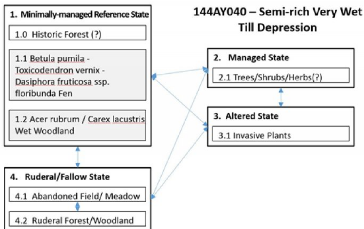
Figure 5. STM_144AY040_Semi-Rich_Very_Wet_Till_Depression
