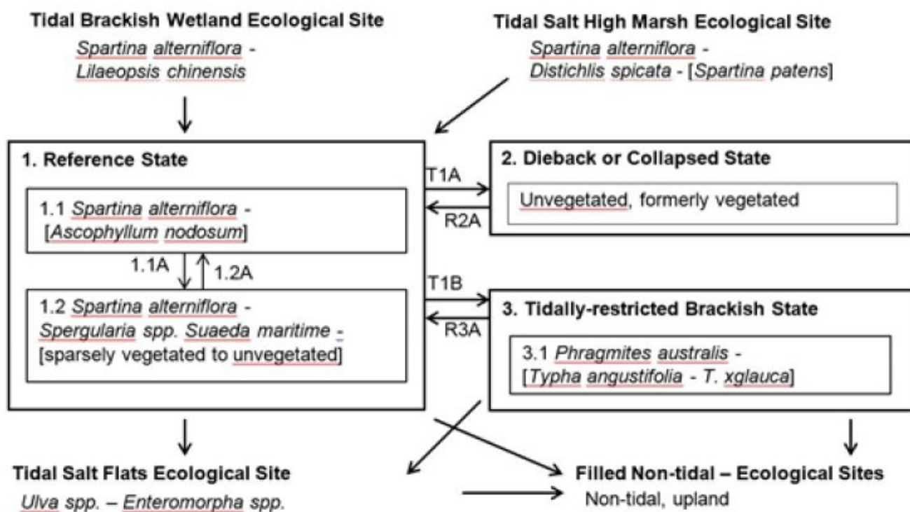
Figure 6. Tidal Salt Low Marsh - R144AR001CT
