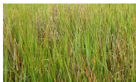
Saltmeadow cordgrass – [knotted wrack] ( Spartina alterniflora – [ Ascophyllum nodosum ])
