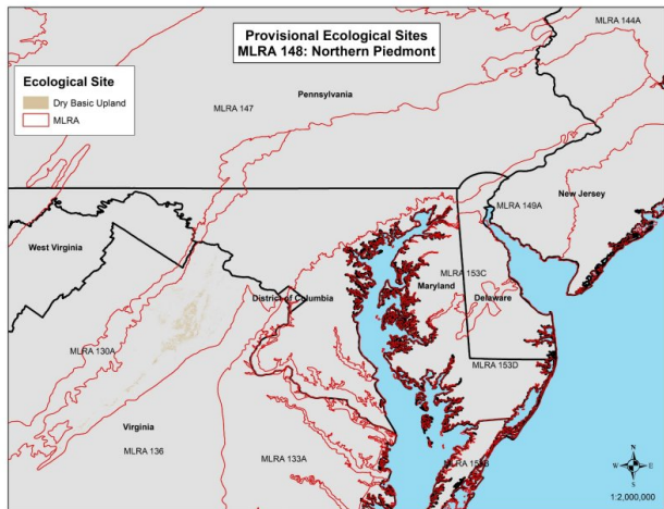
Figure 4. The Dry Basic Upland Ecological Site footprint.
