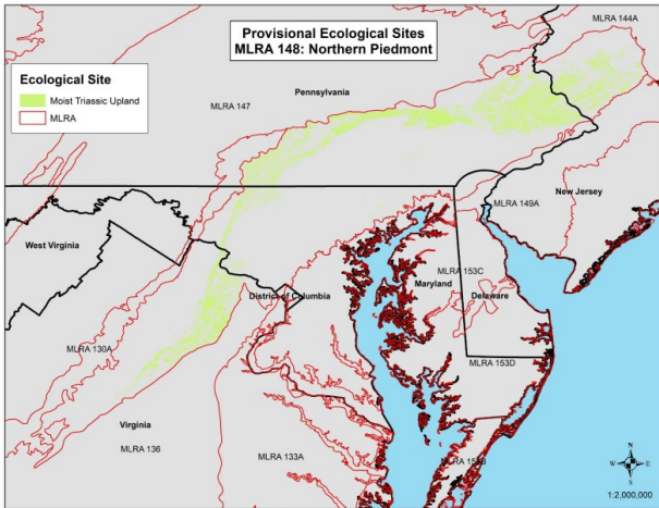
Figure 4. The Moist Triassic Upland Ecological Site footprint.
