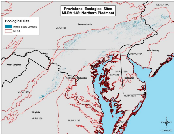
Figure 4. The Hydric Basic Lowland Ecological Site footprint.
