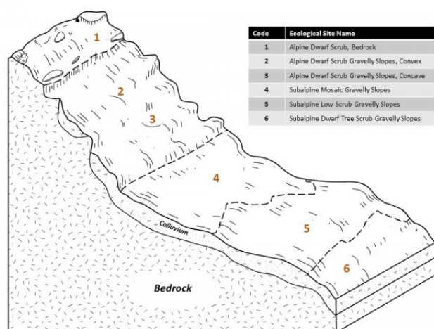
Figure 2. Representative block diagram of Subalpine Dwarf Tree Scrub Gravelly Slopes and associated ecological sites.
