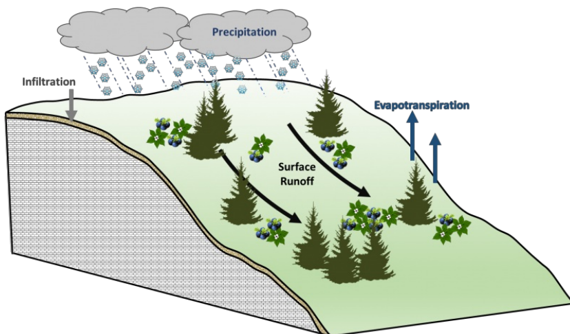
Figure 3. Hydrologic cycling in Subalpine Dwarf Tree Scrub Gravelly Slopes ecological site.
