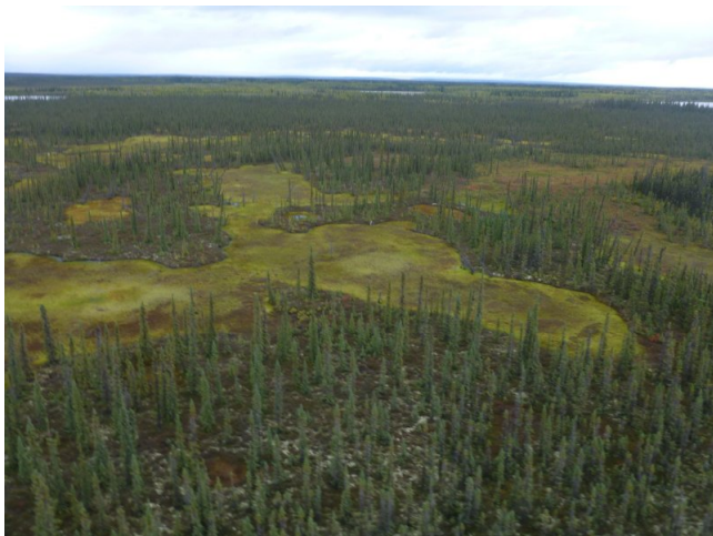
Figure 1. XA232X01Y217 has plant communities associated with thermokarst and floating mat bogs. These bogs are highly acidic and composed primarily of Sphagnum.
