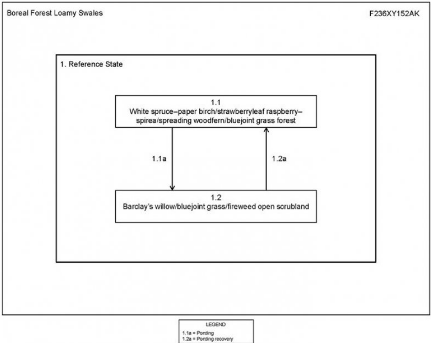
Figure 8. State-and-transition model.
