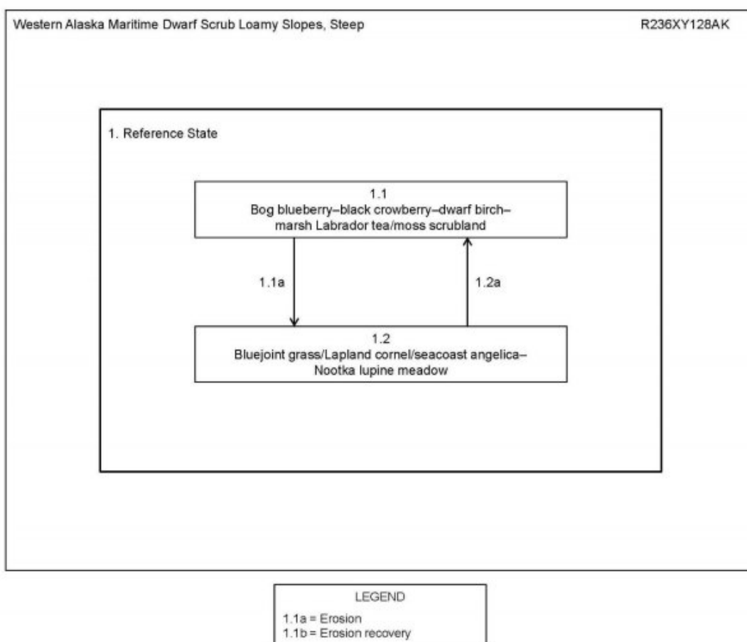
Figure 2. State-and-transition model.
