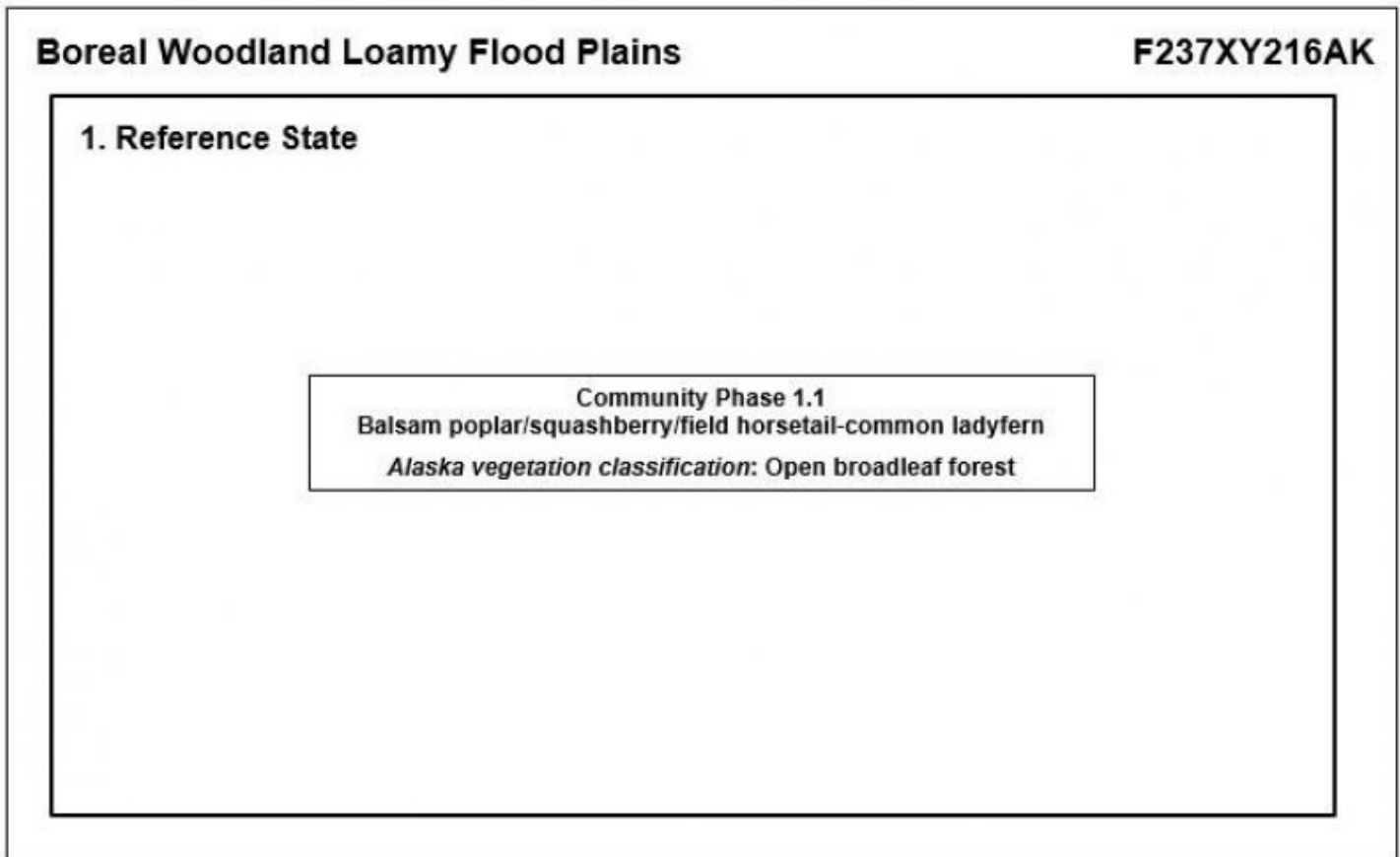
Figure 4. State-and-transition model.
