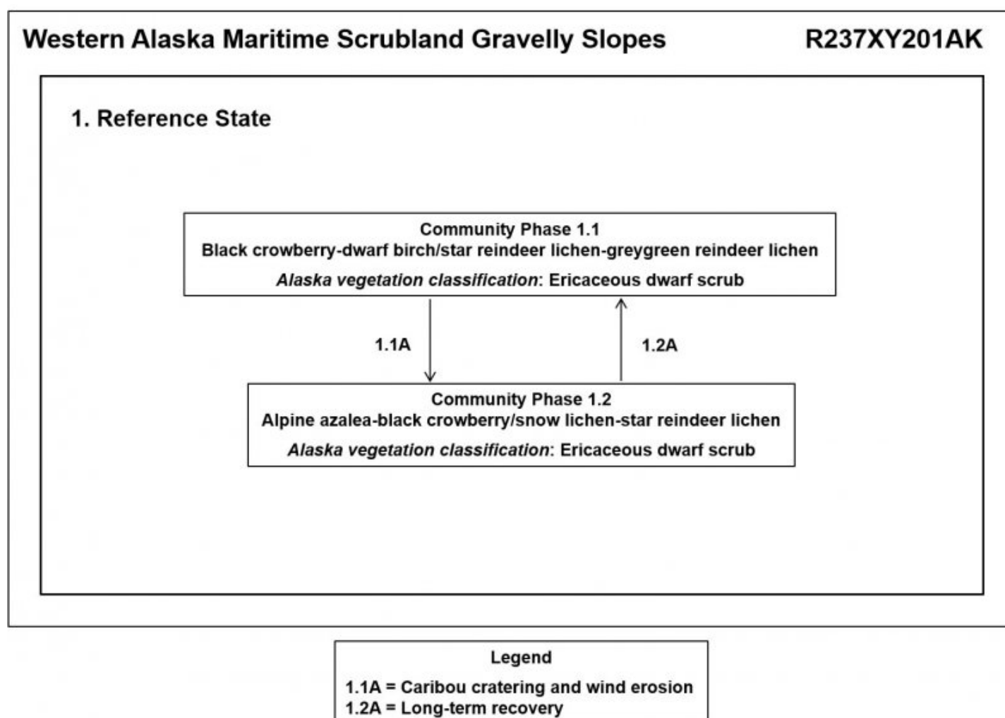
Figure 5. State-and-transition model.
