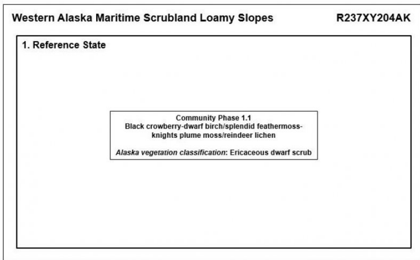
Figure 5. State-and-transition model.
