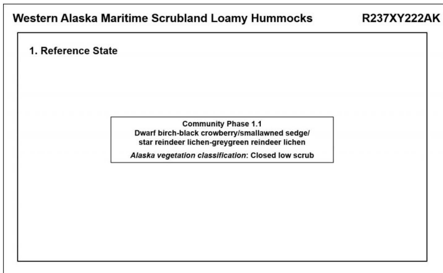
Figure 3. State-and-transition model.
