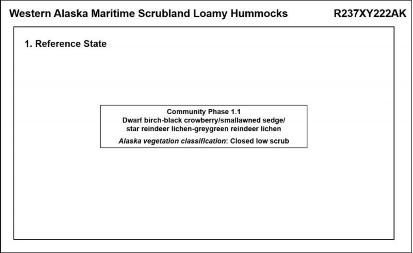
Figure 3. State-and-transition model.
