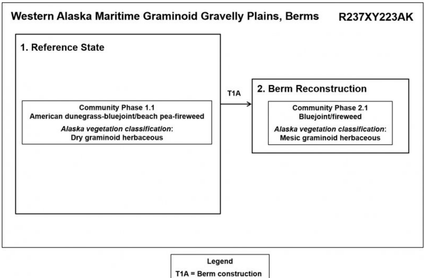
Figure 4. State-and-transition model.
