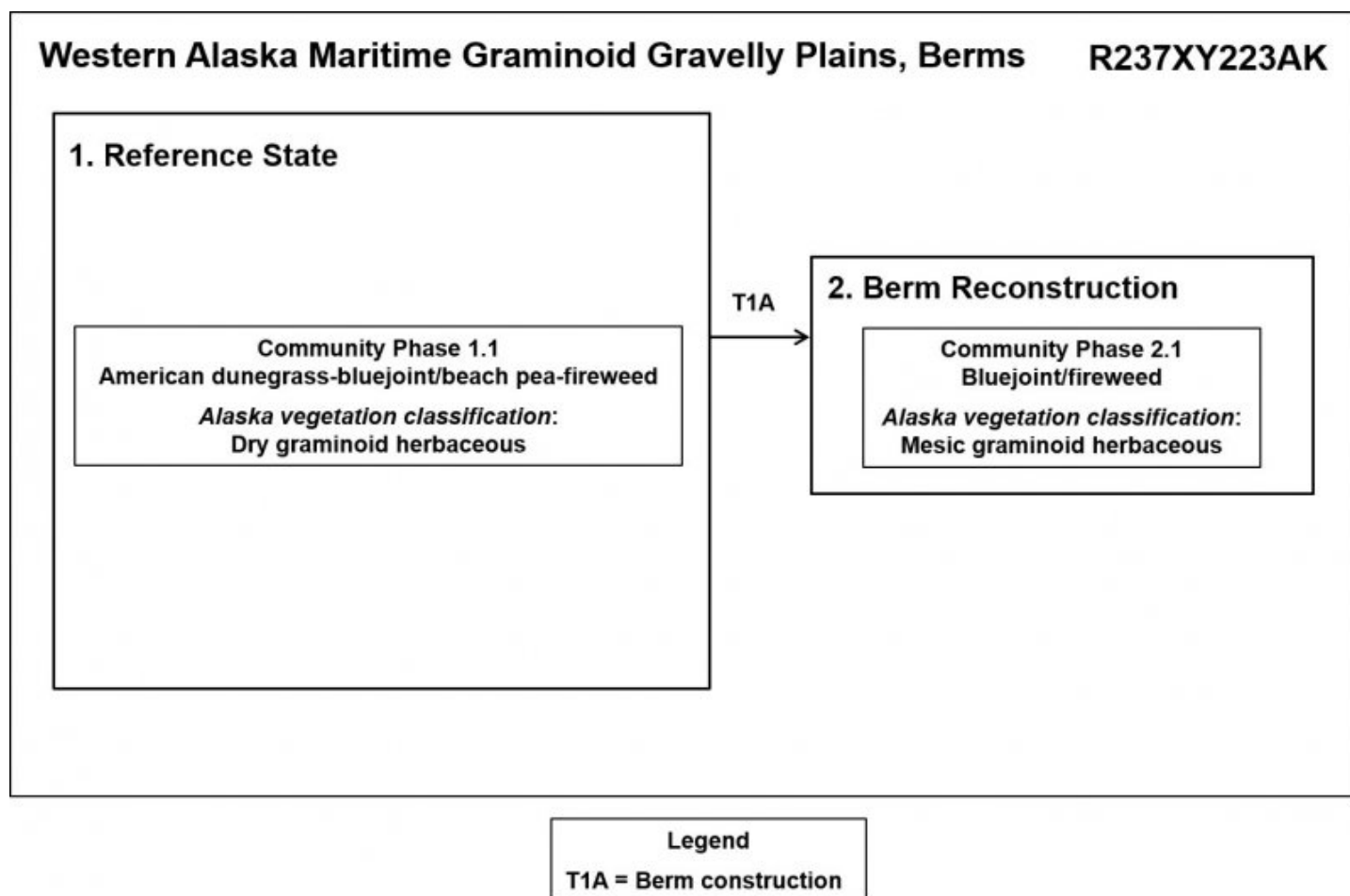
Figure 4. State-and-transition model.
