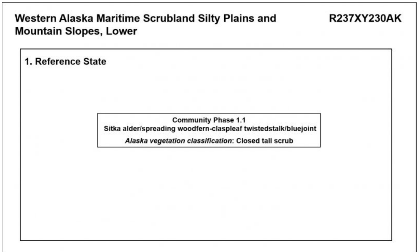
Figure 4. State-and-transition model.
